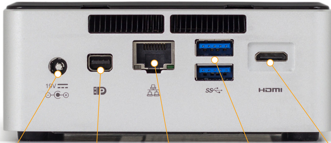
DC Input 19 Volts/3.42 Amps 65 Watts Max
